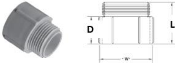
2" through 6" Terminal (Male) Adapter
