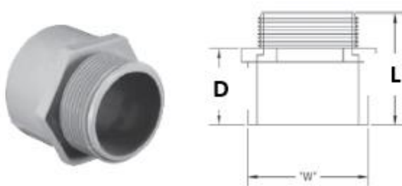
1" through 1 1/2" Terminal (Male) Adapter
